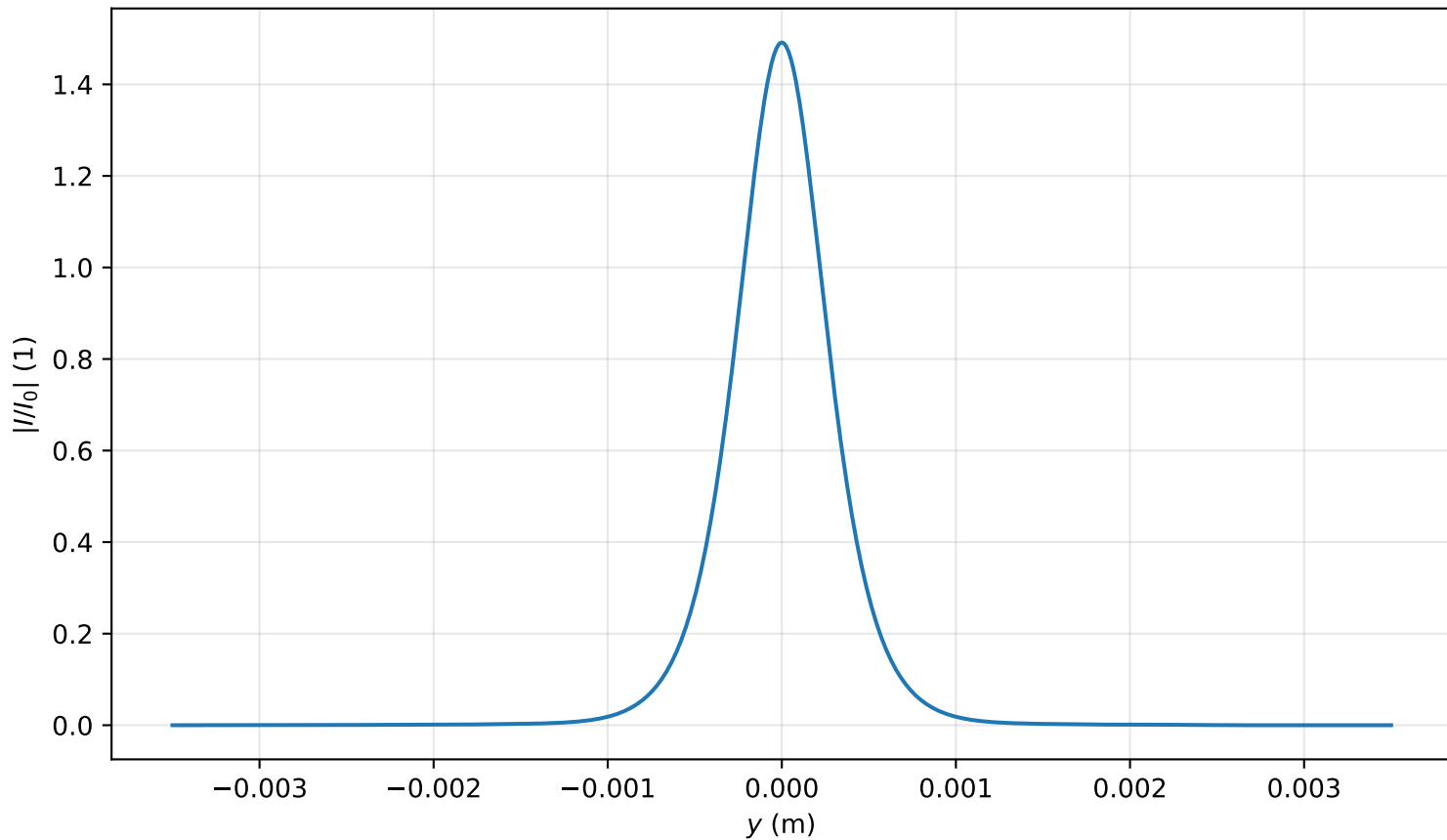
Intensity profile I(x=0, y, z=3.503)/I_0 , P_{in}=0.9P_{cr} , artificial time
